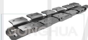
垃圾处理设备用链条 Chains for garbage disposal equipment
