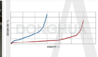
链条磨损曲线 Chain wear elongation curve
